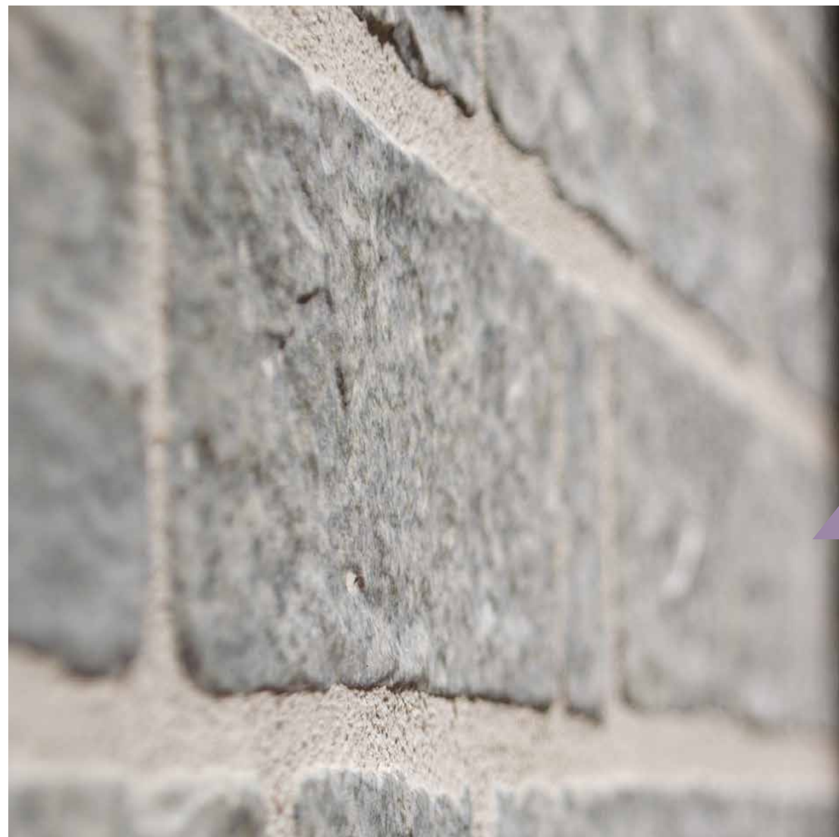
Wall Tile: 22,5x22,5 . 9"x9" Pietra Luserna GRIP / 22,5x45 . 9"x18" Pietra Luserna Ret GRIP Floor Tile: 30x60 . 12"x24" Ret - GRIP
